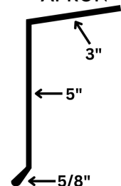
COMMERCIAL GUTTER APRON
