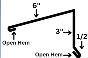
FF100 VENTED J CLEAT
