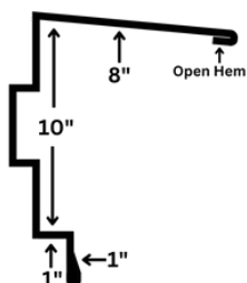
SS200 JAMES ST HIGH SIDE EAVE
