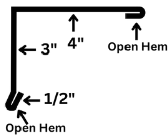
FF100 LOWER GAMBREL
