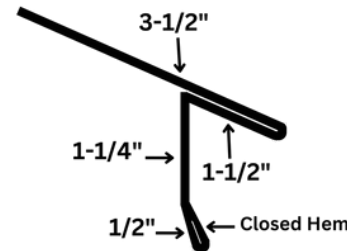
FF100 WIDE VALLEY
