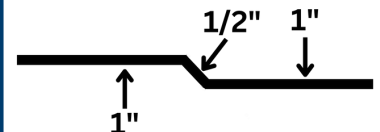
FF100 VALLEY CLEAT
