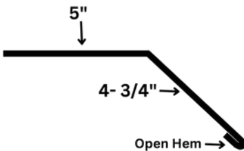
FF100 UPPER GAMBREL
