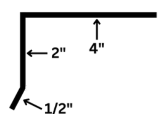
FF100 CHOICE RAKE CLEAT
