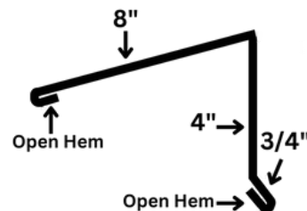
SS200 SIDE WALL
