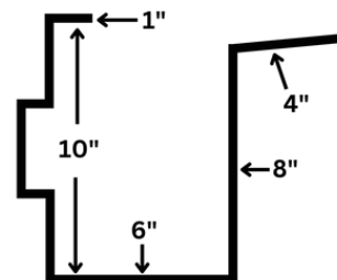
SS200 JAMES ST GUTTER PRE HUNG
