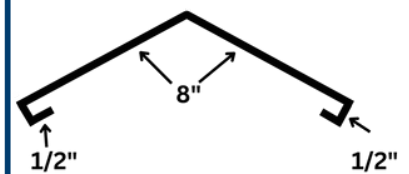
FF100 VENT RIDGE CAP
