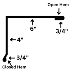
SS200 RIDGE CAP
