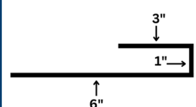
FF100 DEEP J CLEAT
