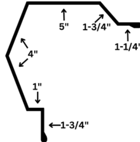
COMMERCIAL PRE HUNG GUTTER
