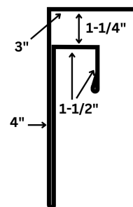
PBR PANEL GUTTER HANGER
