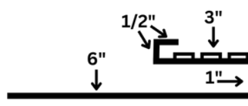
FF100 VENTED J CLEAT
