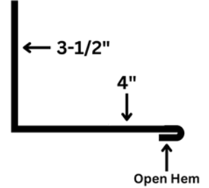
FF100 VENT RIDGE CAP
