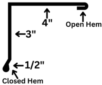
FF100 UPPER GAMBREL
